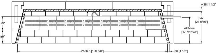
Plan View
