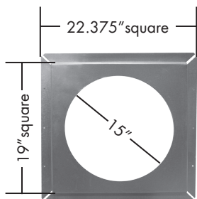
FIRESTOP
