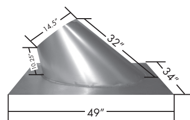
6/12 TO 12/12 FLASHING
