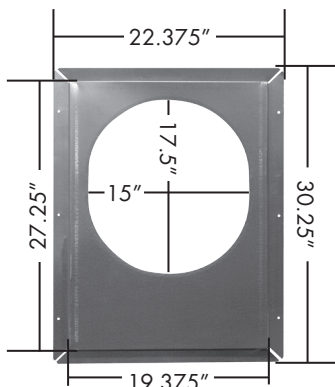
30 DEGREE FIRESTOP
