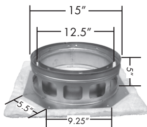
ANCHOR PLATE
