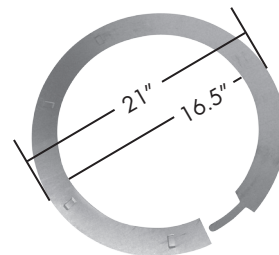
STORM COLLAR
