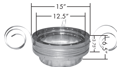
STABILIZER
