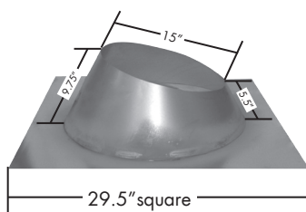
0 TO 6/12 FLASHING
