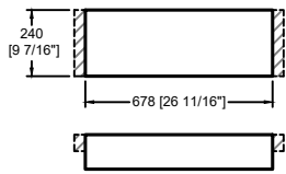
M65a(CC) CUSTOM CUT BACKWALL QTY: 8
