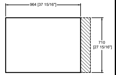
M91a(CC) BASE PLATE QTY: 1
