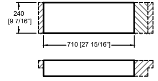
M66a(CC) CUSTOM CUT SIDE WALL QTY: 4
