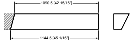
69a(CC) DAMPER BEAM QTY: 2
