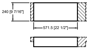
M65b(CC) CUSTOM CUT BACKWALL QTY: 4
